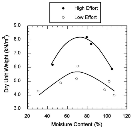
Fig. 3. Compaction data from field test plots
