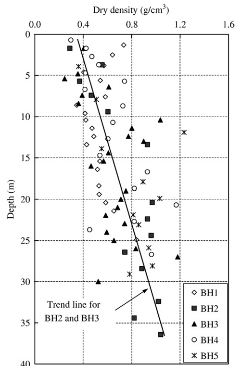
Fig. 5. Variations in dry density with the embedment depth.
