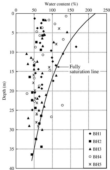
Fig. 11. Variations in water content with the embedment depth.
