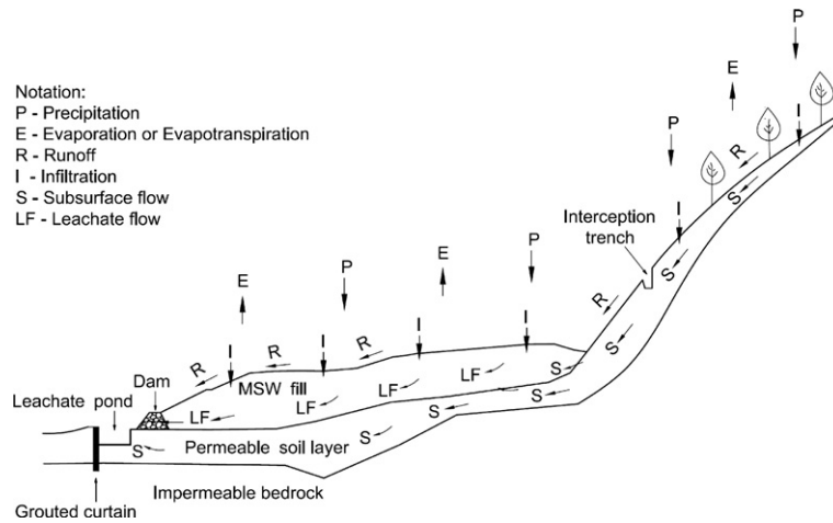
Fig. 10. A schematic diagram showing the hydrogeology system in the Suzhou landfill.
