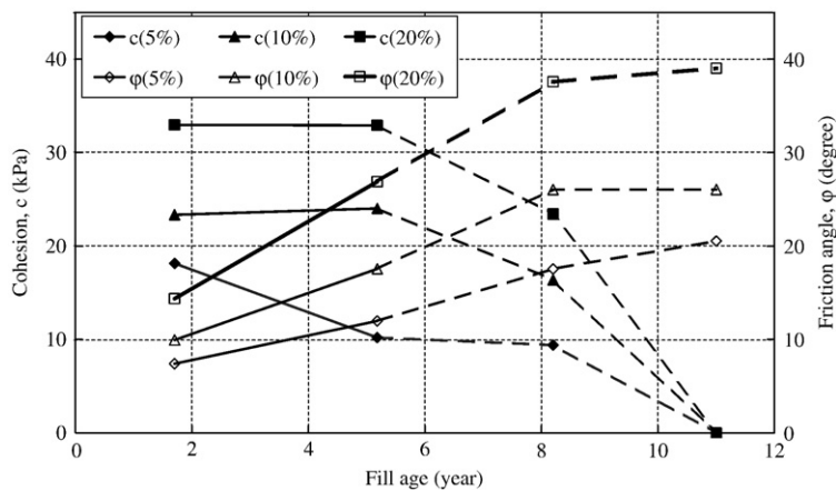
Fig. 8. Relationships of mobilized shear strength parameters at a range of strains to the fill age of MSW (notes: the data points connected by the dashed lines were obtained from samples with different original waste compositions).
