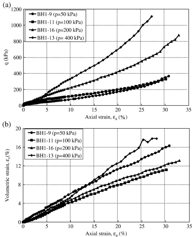
Fig. 6. Stress–strain relationships obtained from four samples with a fill age between 6.8 and 9.3 years: (a) q – \epsilon_a ; (b) \epsilon_v – \epsilon_a .
