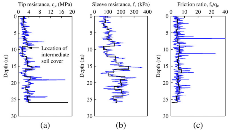
Fig. 13. Results of cone penetration tests from J1.
