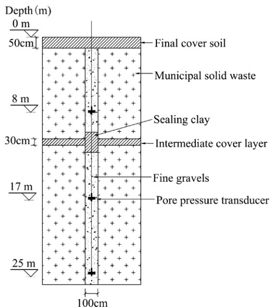
Fig. 2. Layout of pore pressure transducers in boreholes BH1 and BH3.
