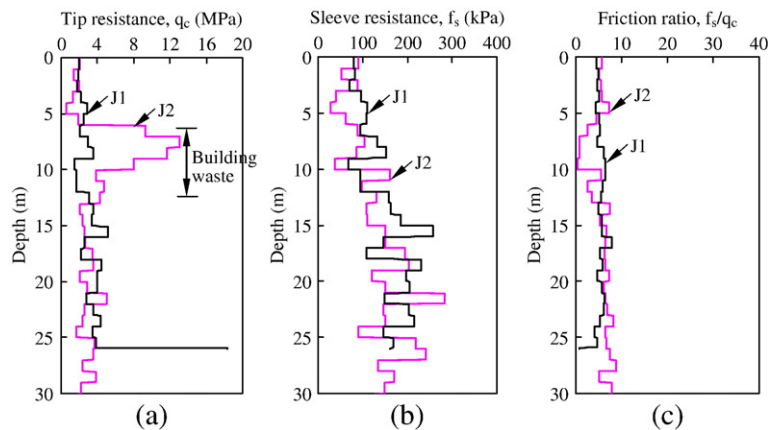
Fig. 14. Comparison of cone penetration test results between J1 and J2.
