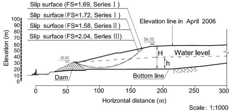
Fig. 15. Results of slope stability analyses on the Suzhou landfill.
