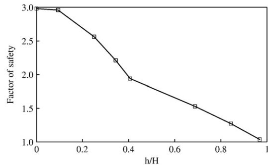
Fig. 16. Influence of leachate level on the slope stability of the Suzhou landfill.
