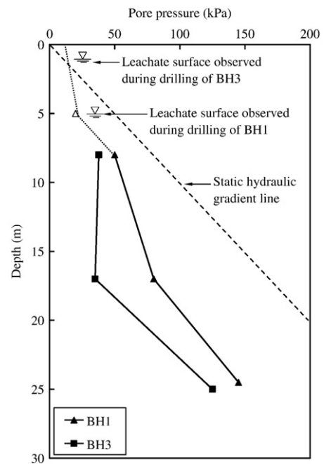
Fig. 12. Profiles of pore pressure measured in boreholes BH1 and BH3.
